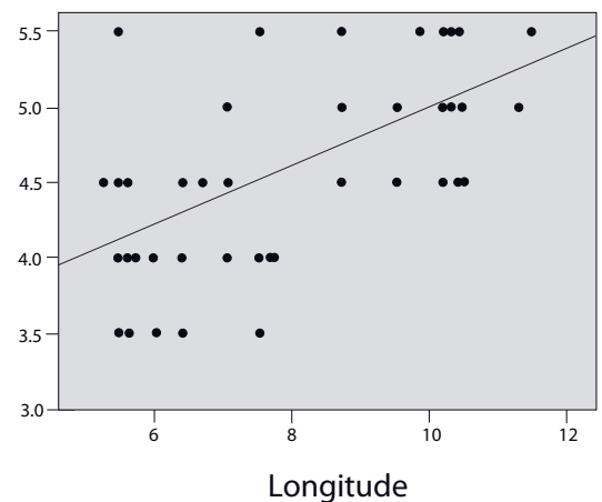
Figure 3. Relationship between the darkness of the mantle colour of the Willow Tits ( n=86 ) and the longitude ( ^{\circ}E ) of sampling sites ( r_s=0.58 , p<0.001 , b_1=0.215 ).
